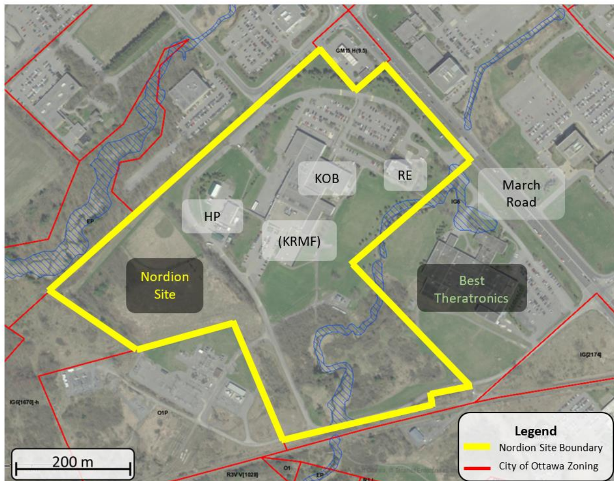
Figure 2: Site Plan
